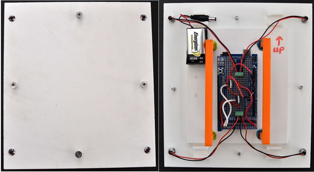
Fig. 1 LED calibration pattern front (left), and LED calibration back: circuitry and battery (right)
