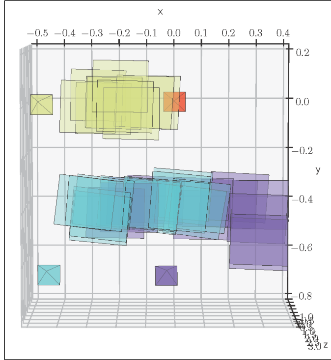
Fig. 7 Calibration pattern poses for each pair of stereo calibrations from Z-axis perspective using extrinsic parameter data extracted using the event-based detection method. Each pattern is colored with respect to the pair: yellow = TL/TR pair, blue = BR/TR, and purple = BL/TR.
