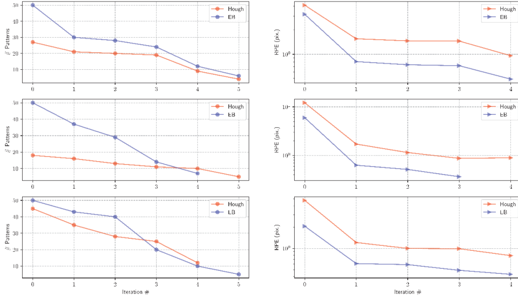
Fig. 6 Stereo calibration algorithm convergence results for the three stereo pairs. Top, middle, and bottom rows correspond to TL/TR (290–291), BR/TR (289–291), and BL/TR (288–291) pairs, respectively. The first and second columns correspond to the number of patterns used for calibration and median RPEs, respectively.
