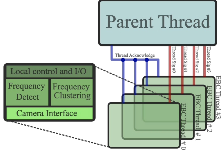
Fig. 3 Structure of multithreaded pattern capture. Each child thread (green) interfaces with an EBC via USB serial connection. It then performs frequency detection algorithms locally before signaling to the parent thread (red). The parent thread (cyan) coordinates parallel capture of the patterns via the thread acknowledge (blue) and terminates the program upon successful registration of the images.
