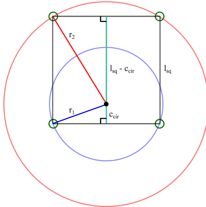
Fig. A-1 Geometric diagram used to derive the parameters for rotating disk design
