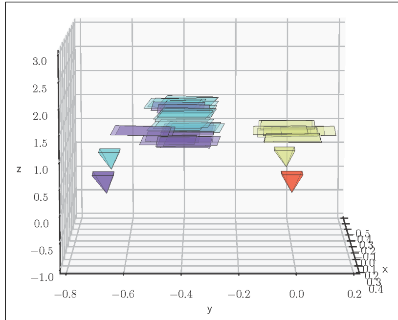
Fig. 8 Calibration pattern poses for each pair of stereo calibrations from X-axis perspective using extrinsic parameter data extracted using the event-based detection method. Each pattern is colored with respect to the pair: yellow = TL/TR pair, blue = BR/TR, and purple = BL/TR.
