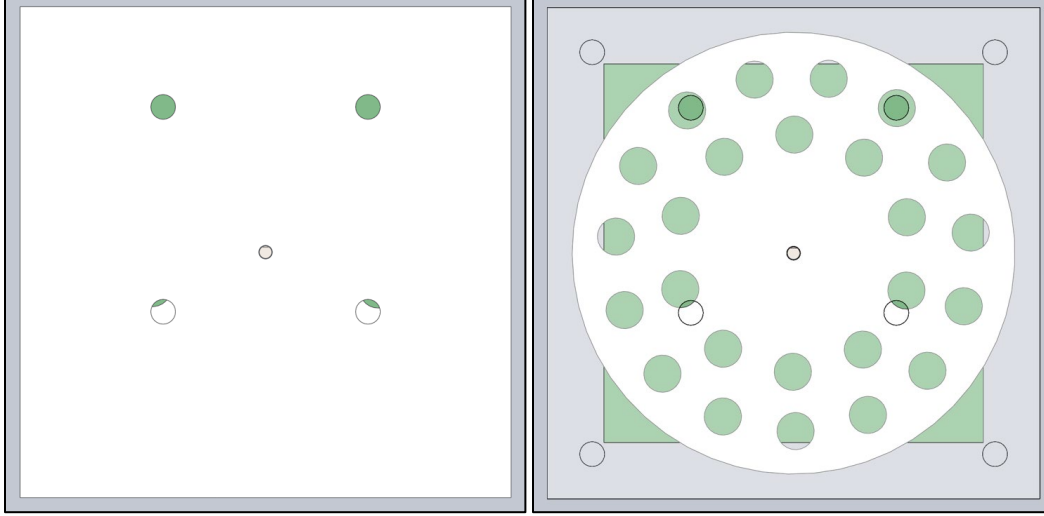
Fig. 2 Rotating disk 3D design: first layer with square dot pattern (left) and second layer with two concentric dotted circles and third layer of reflective material (right)
