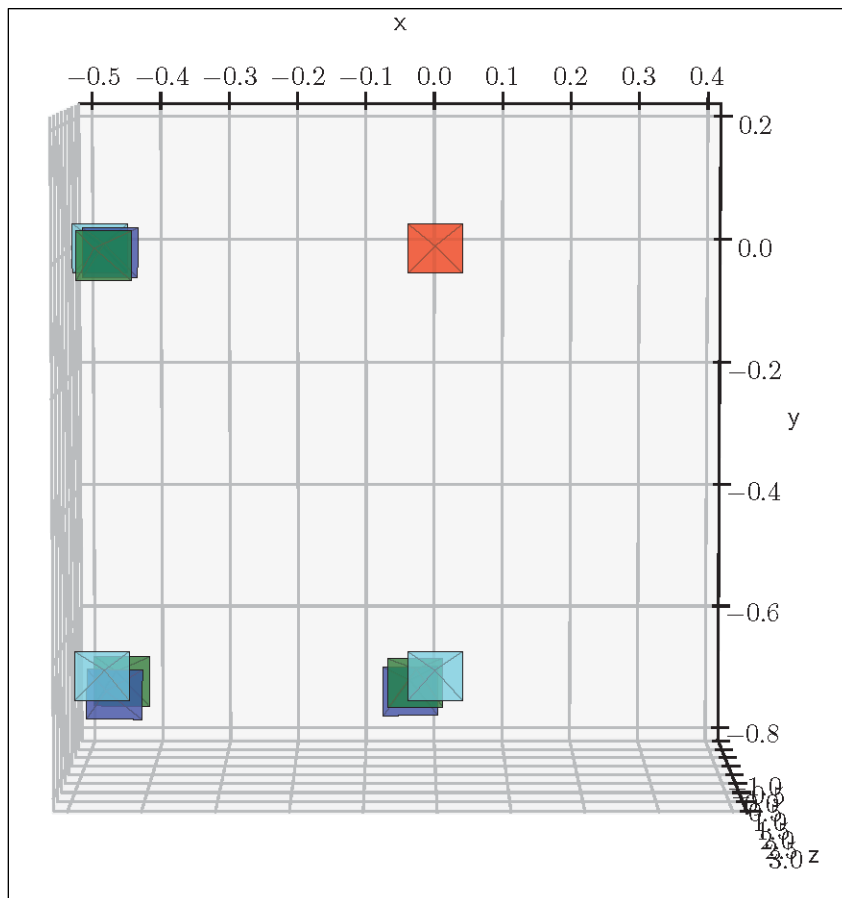
Fig. 9 Camera positions computed from the stereo calibration algorithm with respect to ground truth (cyan). Green and blue camera pyramids correspond to extrinsic parameters extracted using the event-based and Hough transform detection methods, respectively.
