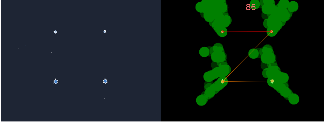
Fig. 4 EBC registration of LED calibration pattern (left) and Metavision intrinsic calibration routine with pattern pose and past patterns embedded (right)
