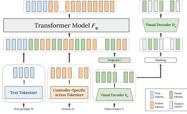
Figure 3. Our unified tokenization framework. We propose a general pre-training strategy for predicting input tokens. For text tokens, we use the standard language modeling task with next token prediction. For actions, we expand the vocabulary of the language model to include action and state tokens that represent each of the action and states possible for the agent across each specific domain. Finally, we incorporate visual tokens into our framework by training a visual encoder-decoder to predict masked visual tokens. F_\phi is trained via causal masking over the entire input sequence S .
