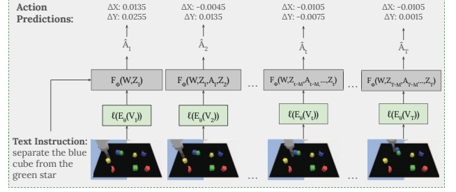
Figure 4. Our robotics and gaming pre-training pipeline. For consistency, we use the same notation as in Sections 2.1 and 2.2; we represent our text instruction as W , input frames as V_t , our visual encoder and linear projection layer as E_\theta and \ell , respectively, our action and language decoder model as F_\phi , and the predicted actions at time step t as \hat{A}_t . In the figure above, we show an example prompt and action prediction set from Language Table, but note that our process is identical across all pre-training datasets.
